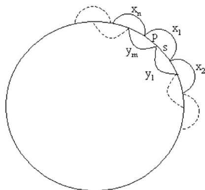
Fig. 1. A graphical representation of the circular code definition. A set of words X is a circular code if any word generated by a concatenation of words of X and written on a circle has a unique decomposition into words of X .
