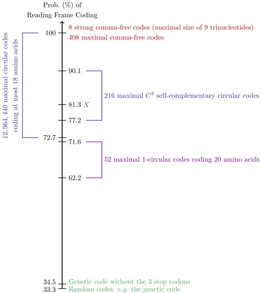
Fig. 6 A probability hierarchy of reading frame coding within two successive codons with the circular (4-circular) trinucleotide codes and the 52 maximal 1-circular trinucleotide codes coding the 20 amino acids (updated from Michel 2014, Fig. 1)
