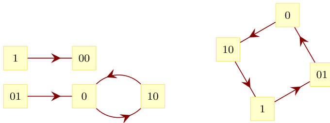
Fig. 8 Graphs \mathcal{G}(Y_1) (left) and \mathcal{G}(Y_2) (right)
