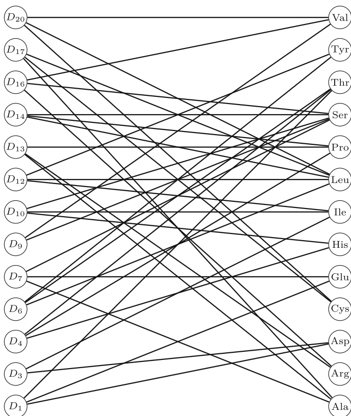
Fig. 5 Bipartite graph \mathcal{G} = (V, E) where V is composed of the 13 equivalence classes in D = \{D_1, D_3, D_4, D_6, D_7, D_9, D_{10}, D_{12}, D_{13}, D_{14}, D_{16}, D_{17}, D_{20}\} and the 13 amino acids in A = \{\text{Val, Tyr, Thr, Ser, Pro, Leu, Ile, His, Glu, Cys, Asp, Arg, Ala}\} , and E is the set of all pairs (D_i, aa) such that there is a codon in D_i that encodes the amino acid aa
